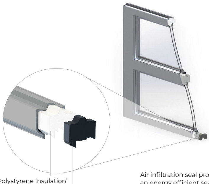
Stylist Cross Section* *Pictured with optional insulation
